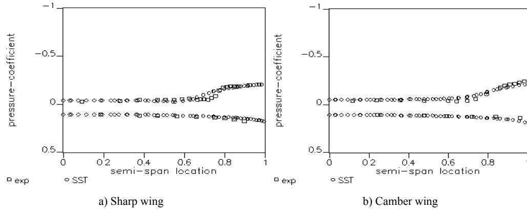
Fig. 8. Comparison of Co-efficient of pressure of two wing profiles with SST Turbulence model and co-relation with experimental data at M=1.6 \alpha= 5.25^\circ (sharp wing) and \alpha= 5.17^\circ (camber wing), Re= 2 \times 10^6 at Z/C_R=0.33
