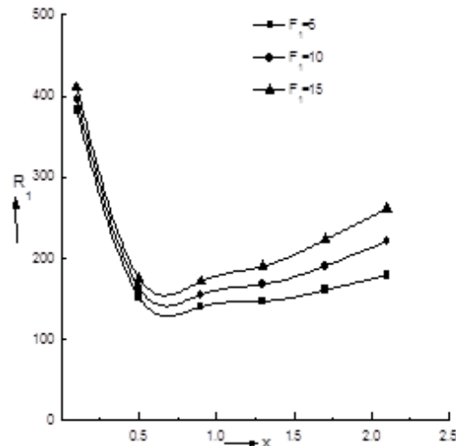
Fig.4. The variation of Rayleigh number R_1 with x for S_1=10, Q_1=20, P=5, T_1=200, F_1=5,10 and 15 .
