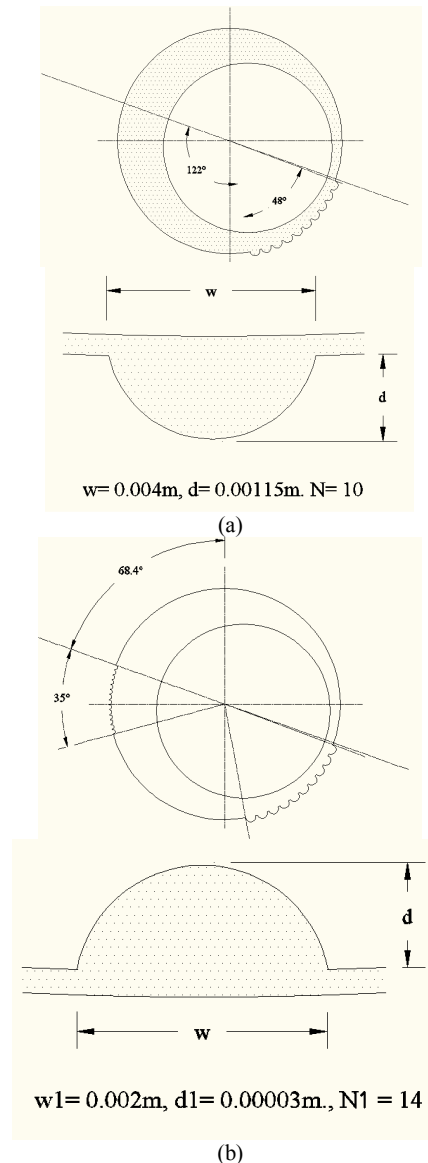
Fig. 1. Two-dimensional model: (a) textured bearing model and (b) dimple geometry
