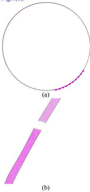
Fig.4. (a) and (b) meshed view of modified dimpled bearing in Fluent 6.3.26 have been shown.
