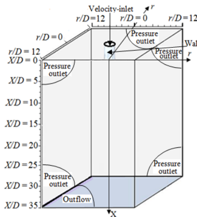
Fig. 5. Calculation domain and working stress.
