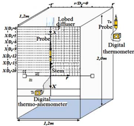
Fig. 1. Schematic description of the experimental installation.
