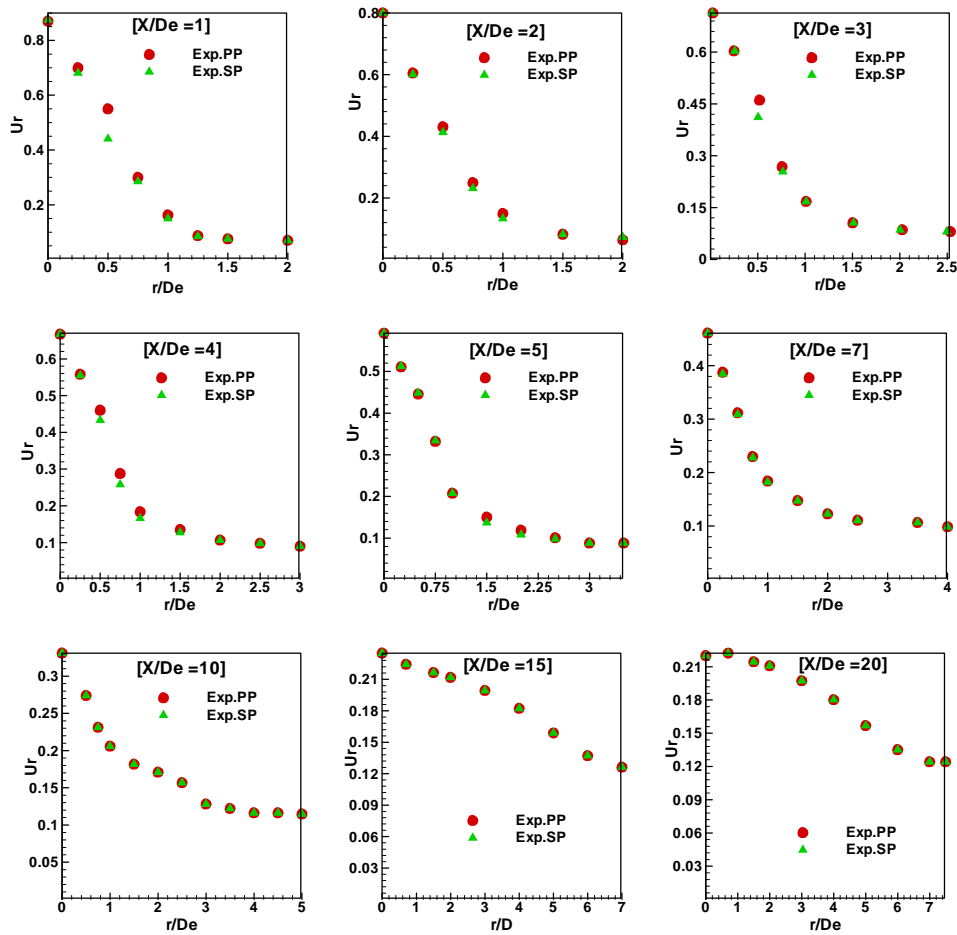
Fig. 4. Radial velocity profiles of a free lobed jet.
