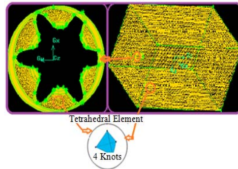
Fig. 6. Meshing of the calculation domain.
