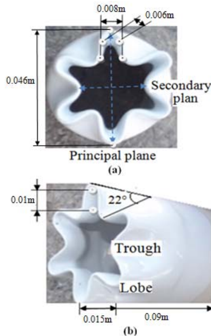
Fig. 2. “a), Geometry of the blowing plane (YZ),”b) Photography of a lobed nozzle.
