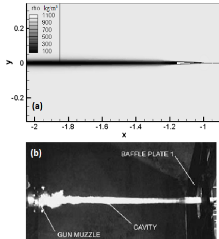
Fig. 13. (a) Simulated supercavitation profile behind the projectile (b) The experimental shape of supercavitation profile behind the projectile.
