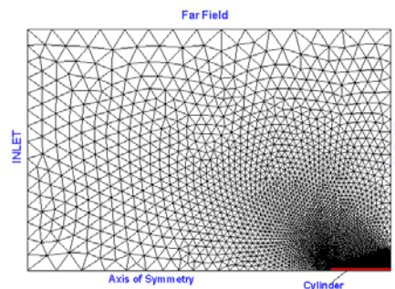
Fig. 6. Computational domain and boundary conditions.
