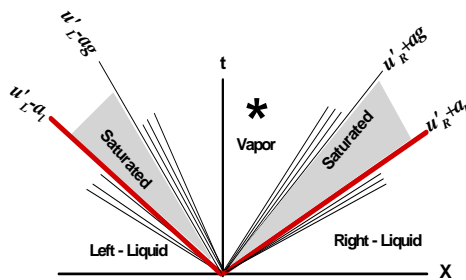
Fig. 2. Wave pattern in the Riemann problem.
