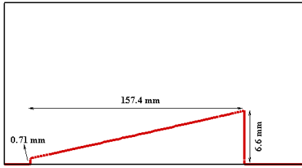
Fig. 9. Schematic shape of the projectile with the apex angle of 2.1^\circ .
