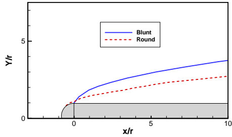
Fig. 21. Cavitation profile around the cylinder with blunt and round head.
