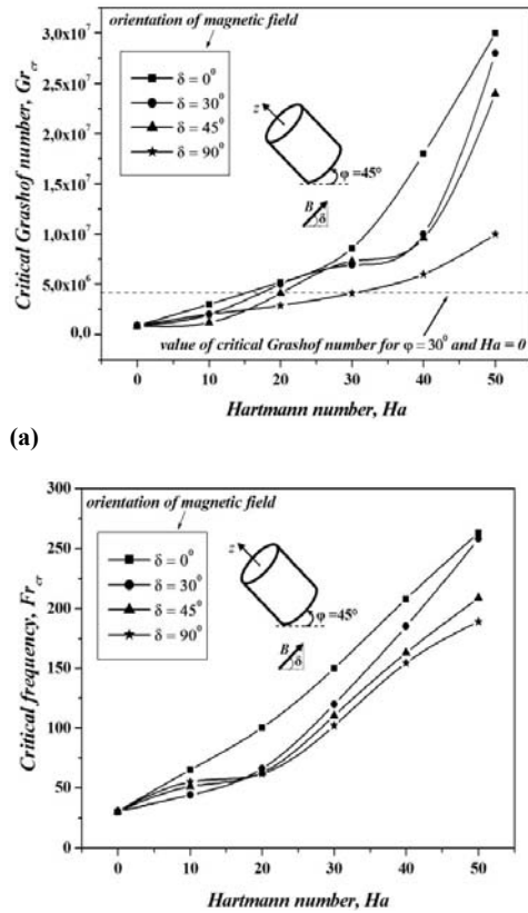
Fig. 11. Magnetohydrodynamic stability diagram for different orientation of magnetic field, (a) Gr_{cr} - Ha and (b) Fr_{cr} - Ha . The enclosure has a fixed inclination \varphi = 45^\circ ( Ha \leq 50 ).
