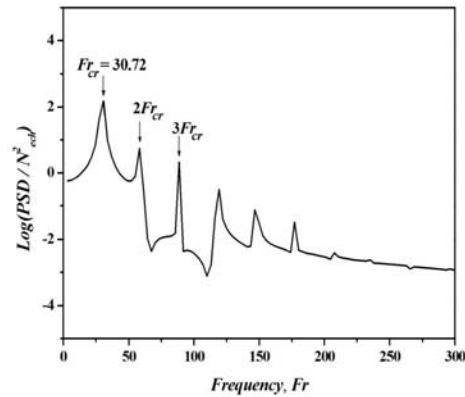
Fig. 5. Power spectrum of the dimensionless radial velocity component u , for Gr_{cr} = 9 \times 10^5 , \phi = 45^\circ and Ha = 0 . Fr_{cr} = 30.72 , represent the dimensionless critical frequency.
