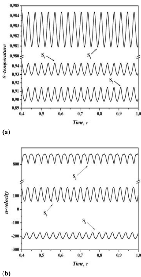
Fig. 4. Time evolution of the dimensionless temperature \theta at S_1 , S_4 and S_7 (a), and dimensionless radial velocity component u at S_2 , S_5 and S_8 (b), for Gr_{cr} = 9 \times 10^5 , \phi = 45^\circ and Ha = 0 .
