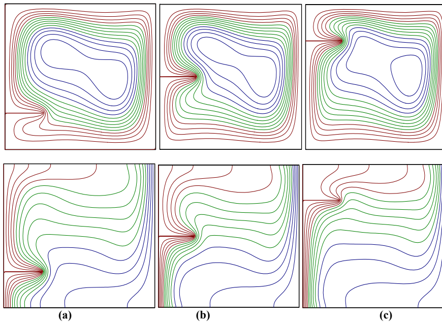
Fig. 5. Effect of baffle position on streamlines (top) and isotherms (bottom) for \epsilon = 0.25 and Ra = 10^5 . (a) L = 0.25 , |\psi_{\max}| = 14.4 , (b) L = 0.5 , |\psi_{\max}| = 13.5 , (c) L = 0.75 , |\psi_{\max}| = 12.6 .
