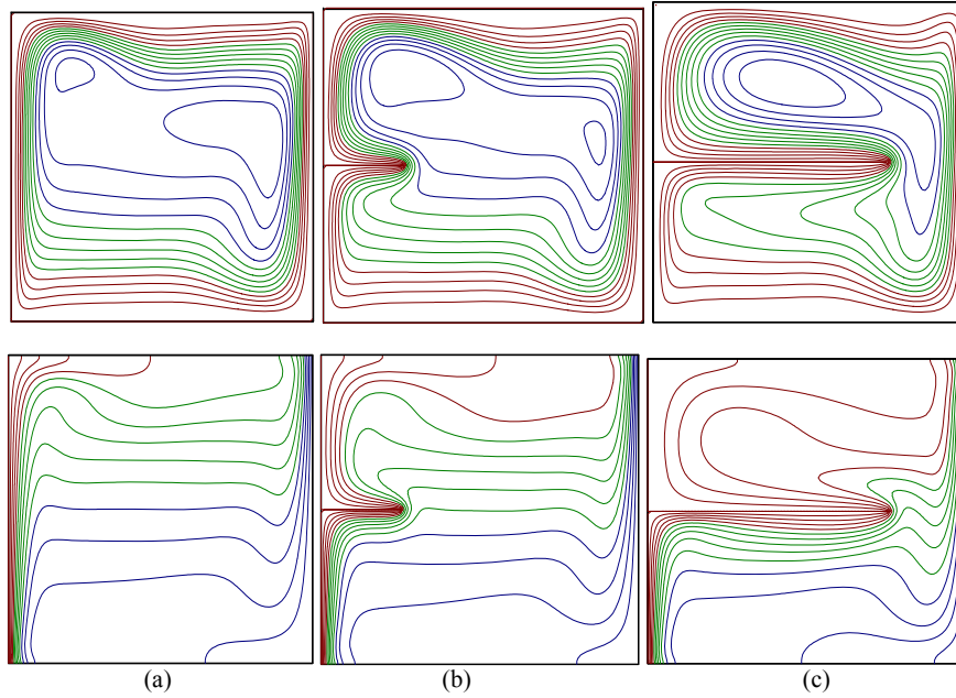
Fig. 4. Effect of baffle length on streamlines (top) and isotherms (bottom) for L = 0.5 and Ra = 10^6 . (a) No baffle, |\psi_{\max}| = 22.9 , (b) \epsilon = 0.25 , |\psi_{\max}| = 27 and (c) \epsilon = 0.75 , |\psi_{\max}| = 34.9 .
