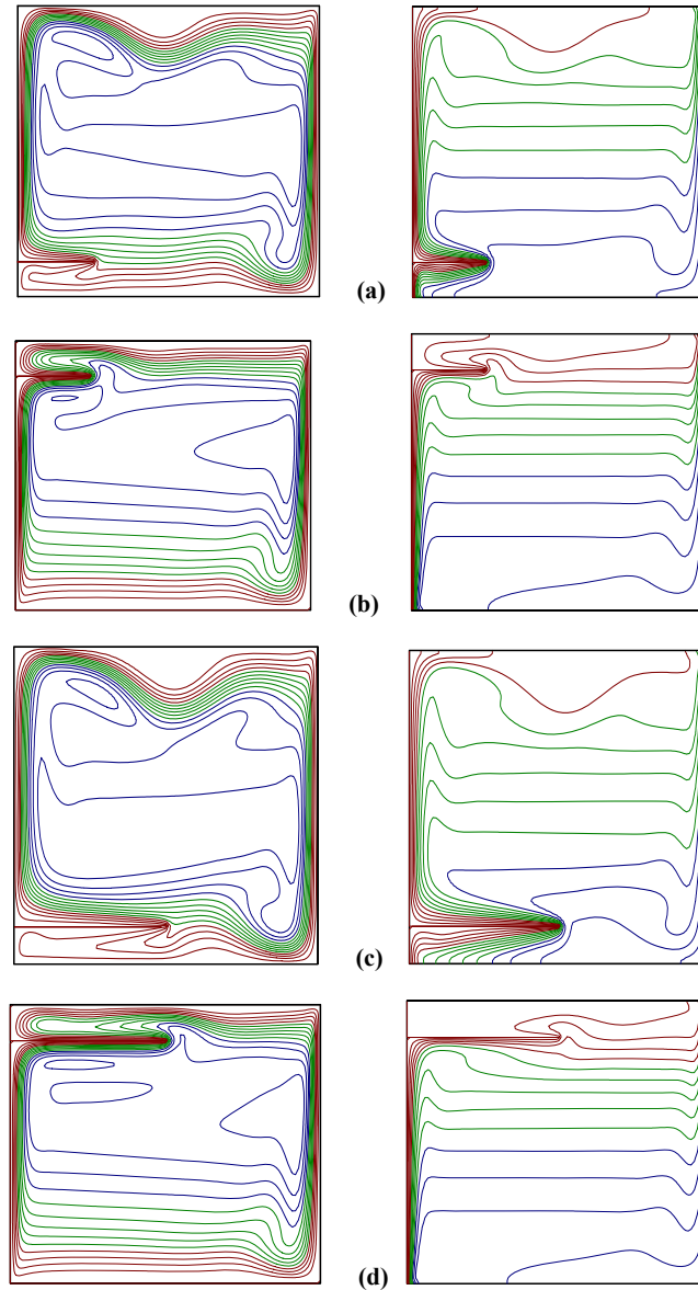
Fig. 6. Streamlines (left) and isotherms (right) for various baffle lengths and positions at Ra = 10^7 . (a) |\psi_{\max}| = 43.9 , (\epsilon, L) = (0.25, 0.125) , (b) |\psi_{\max}| = 37.3 , (\epsilon, L) = (0.25, 0.875) , (c) |\psi_{\max}| = 49.4 , (\epsilon, L) = (0.5, 0.125) , (d) |\psi_{\max}| = 36.6 , (\epsilon, L) = (0.5, 0.875) .
