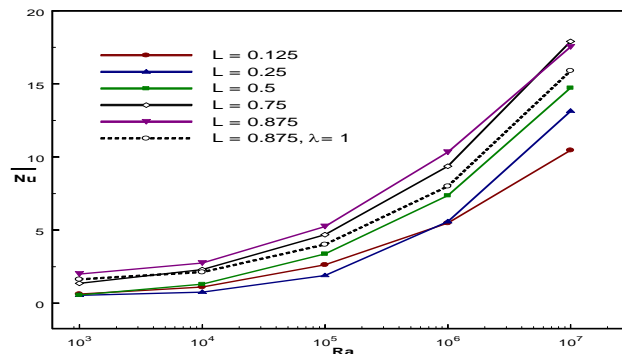
Fig. 9. Effect of baffle position on average Nusselt number for different Rayleigh numbers and \epsilon = 0.5 .
