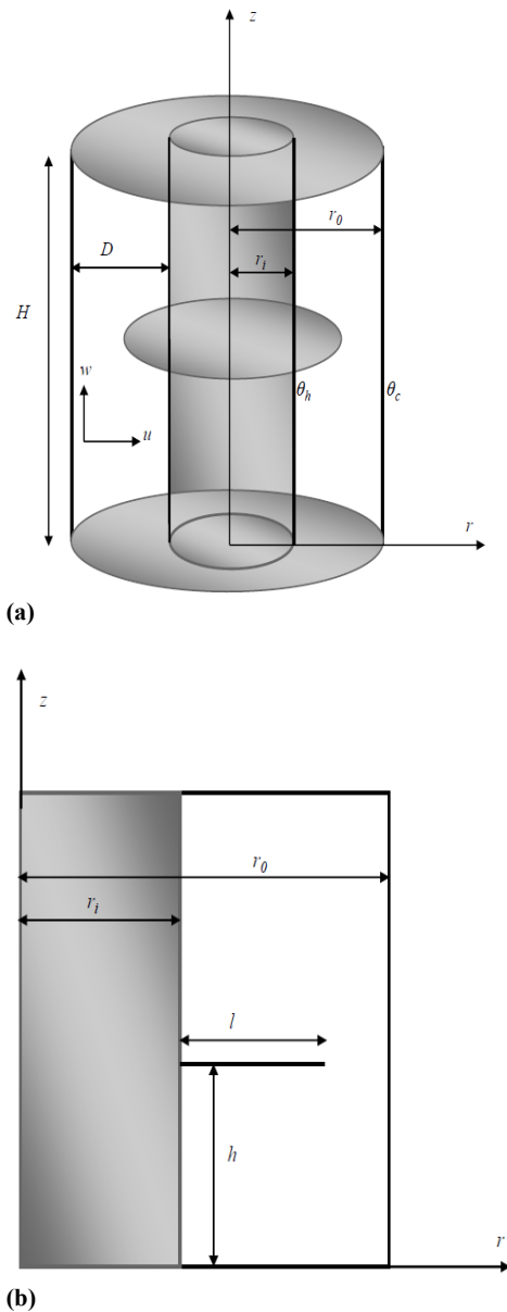
Fig. 1. (a) Physical configuration, co-ordinate system and (b) axisymmetric view of the annulus.
