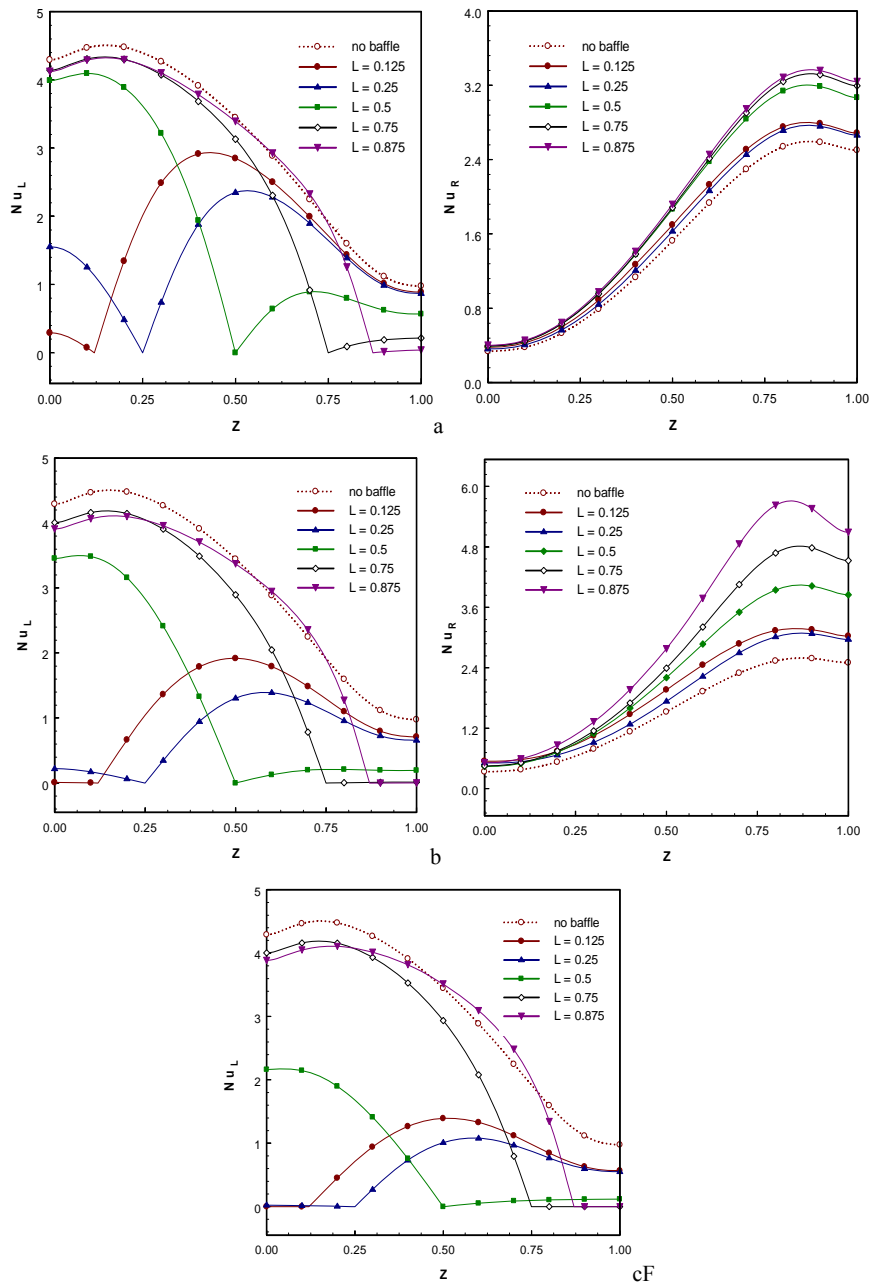
Fig. 7. Variation of local Nusselt number along the inner (left) and outer (right) walls of the annulus for different positions and lengths of baffle at Ra = 10^4 (a) \varepsilon = 0.25 , (b) \varepsilon = 0.5 and (c) \varepsilon = 0.75 .
