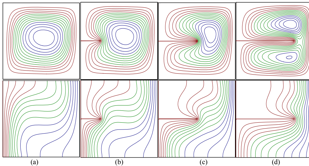
Fig. 3. Effect of baffle length on streamlines (top) and isotherms (bottom) for L = 0.5 and Ra = 10^4 . (a) No baffle, |\psi_{\max}| = 6.7 , (b) \varepsilon = 0.25 , |\psi_{\max}| = 7.4 , (c) \varepsilon = 0.5 , |\psi_{\max}| = 6.8 , and (d) \varepsilon = 0.75 , |\psi_{\max}| = 3.8 .
