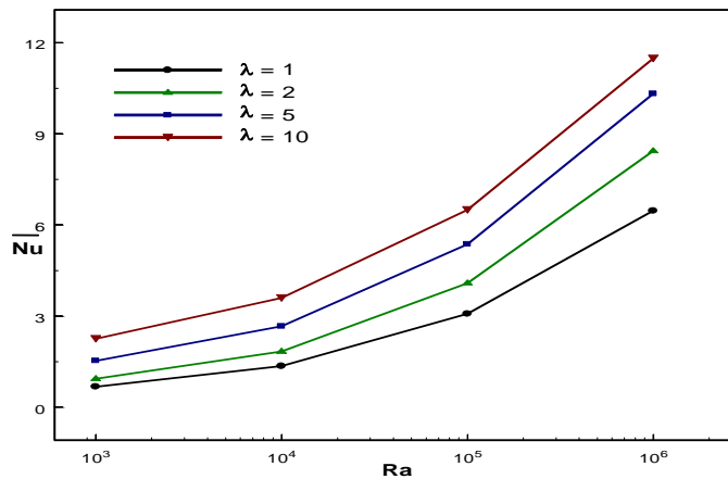
Fig. 10. Effect of radius ratio and Rayleigh number on the average Nusselt number for baffle position L = 0.5 and baffle length \varepsilon = 0.25 .
