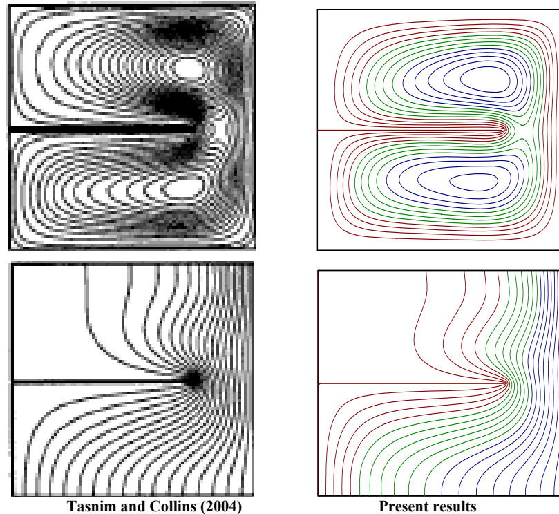
Fig. 2. Comparison of streamlines and isotherms between the numerical results of Tasnim and Collins (2004) and present results for Ra = 10^4 , \lambda = 1 , A = 1 , L = 0.5 , \varepsilon = 0.75 and Pr = 0.7 .
