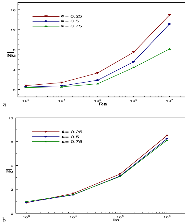
Fig. 8. Effect of baffle length and Rayleigh number on the average Nusselt number for two different baffle positions (a) L = 0.25 and (b) L = 0.75 .
