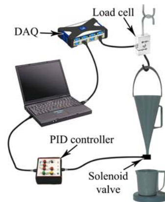
Fig. 2. Experimental setup.
