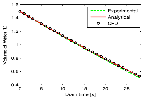
Fig. 5. Draining time as a function of water volume (discharge coefficient c_d=0.895 ).
