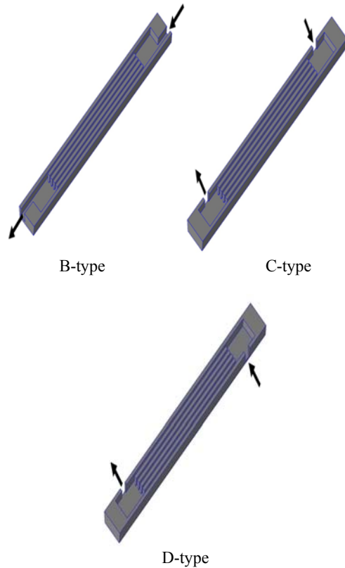
Fig. 3. The geometry showing the B-, C- and D-type entry/exit configurations.
