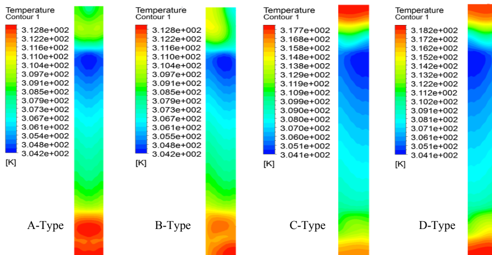
Fig. 12. Temperature distribution of the base plate of MCHS with different entry/exit configurations at \Delta P=15 kPa.
