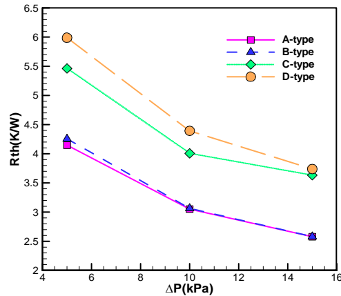
Fig. 14. Variation of thermal resistance with pressure drop for various entry/exit configurations.
