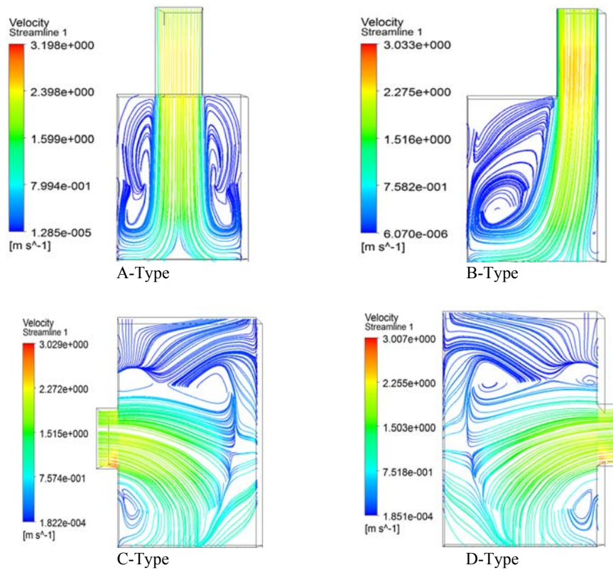
Fig. 9. Streamlines at mid plane of the entry plenum at \Delta P = 15 kPa.
