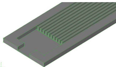
Fig. 4. The geometry of Chein and Chen (2009) and Phillips (1988); utilized here for the validation study.
