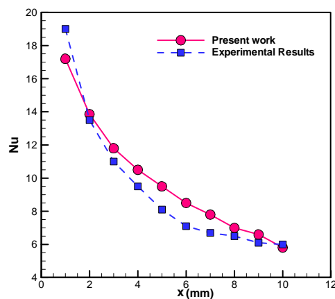
Fig. 6. Variation of local Nusselt number along microchannel #5 in the present study and in the experimental study of Philips (1988) for \Delta P=15 kPa.
