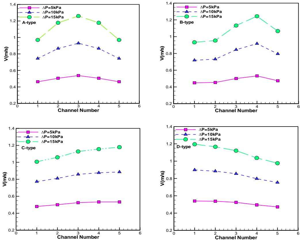
Fig. 8. Average velocity in different microchannels for different pressure drops.
