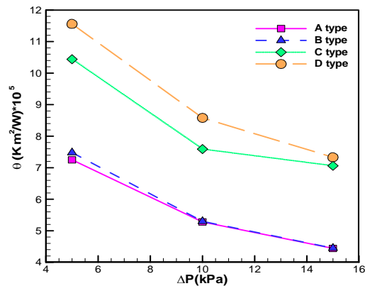
Fig. 15. Variation of theta with pressure drop for various entry/exit configurations.
