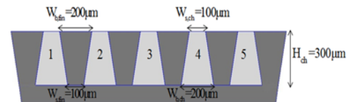
Fig. 2. Fin and microchannel dimensions.
