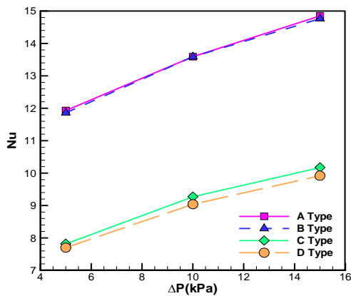
Fig. 13. Variation of average Nusselt number with pressure drop for various entry/exit configurations.
