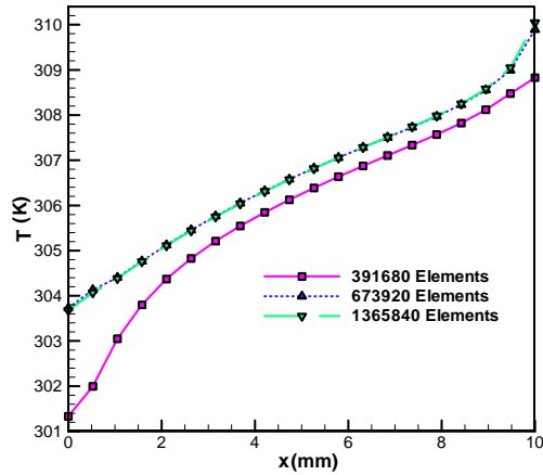
Fig. 7. Temperature along bottom center of microchannel #3 in A-type MCHS using three different grid systems; \Delta P=15 kPa and q_w=200 kW/m 2 .
