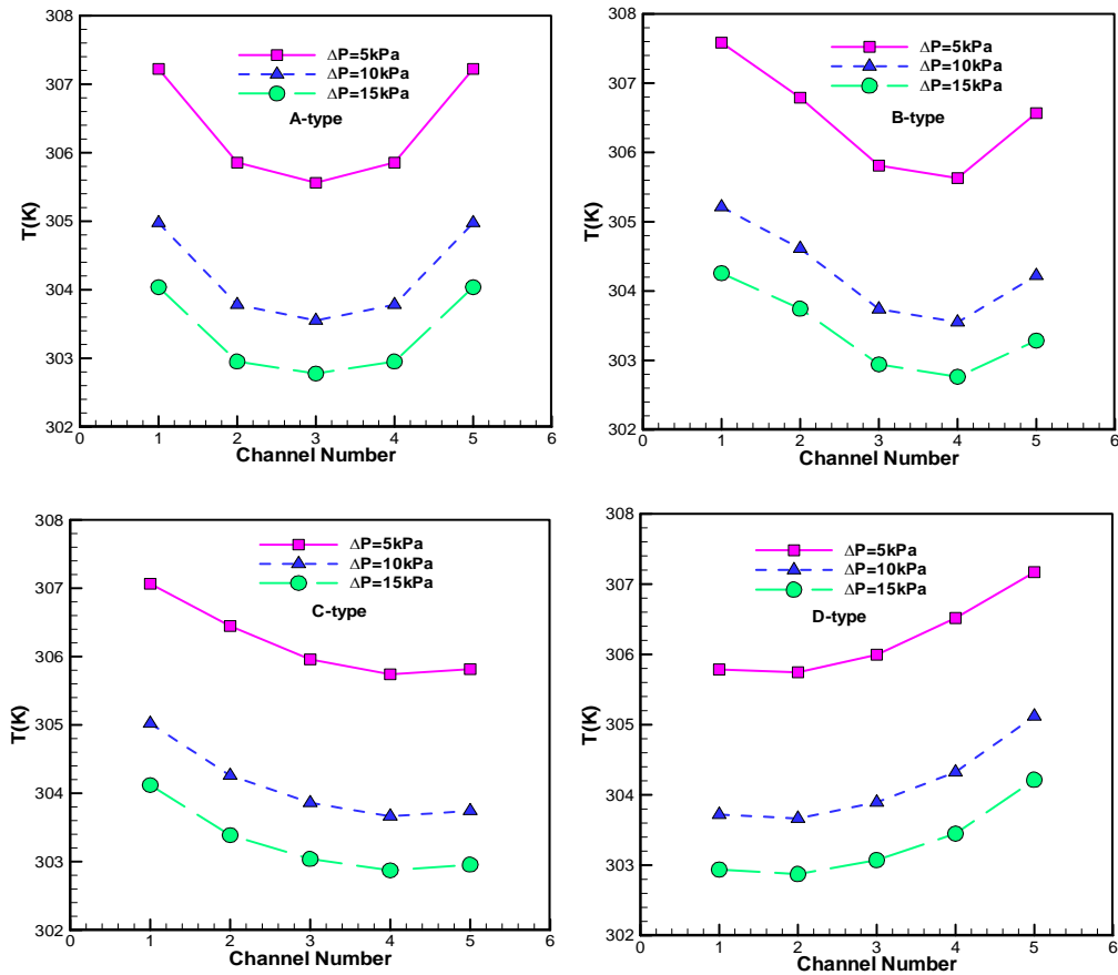
Fig. 10. The flow average temperature in different microchannels.
