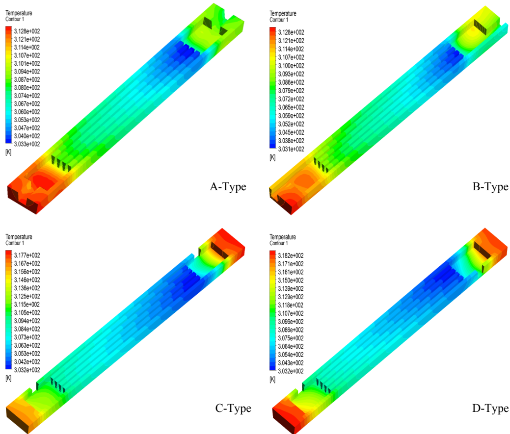
Fig. 11. Temperature distribution in the solid part of MCHS with different entry/exit configurations at \Delta P=15 kPa.
