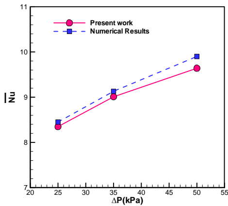
Fig. 5. The average Nusselt number obtained in the present study and that of Chein and Chen (2009) for three pressure drops of 25, 35 and 50 kPa.
