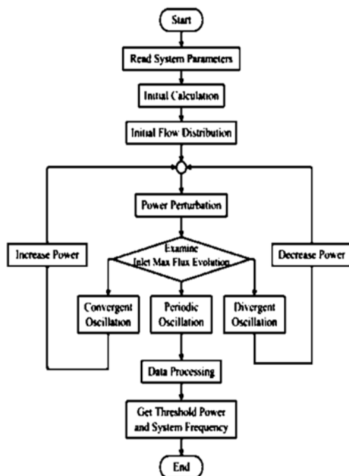
Fig. 3. Calculation algorithm.
