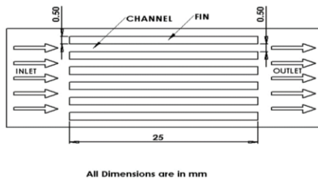
All Dimensions are in mm Fig. 2. Sketch of the plate fin microchannel heat sink.
