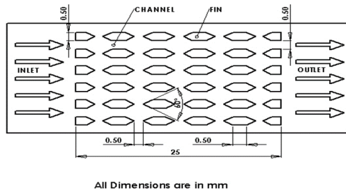
All Dimensions are in mm Fig. 1. Sketch of the modified hexagonal fin microchannel heat sink.
