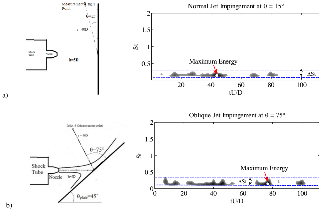
Fig. 11. Scalogram of the acoustic waves for a) normal jet impingement at \theta=15^\circ and b) oblique jet impingement at \theta=75^\circ at the far-field of the impinging point.
