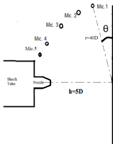
Fig. 9. Position of the microphones for normal jet impingement.
