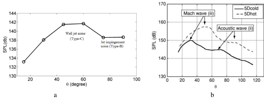
Fig. 7. OASPL of the oblique jet impingement to a 45^\circ inclined plate at different polar angles a) present study b) result of Nonomura, Goto, and Fujii (2011).
