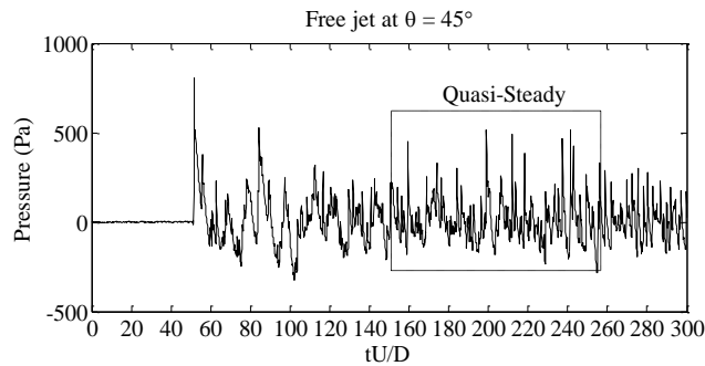
Fig. 3. Acoustic signature of the free jet at \theta = 45^\circ (data from mic.4 in Fig. 2).
