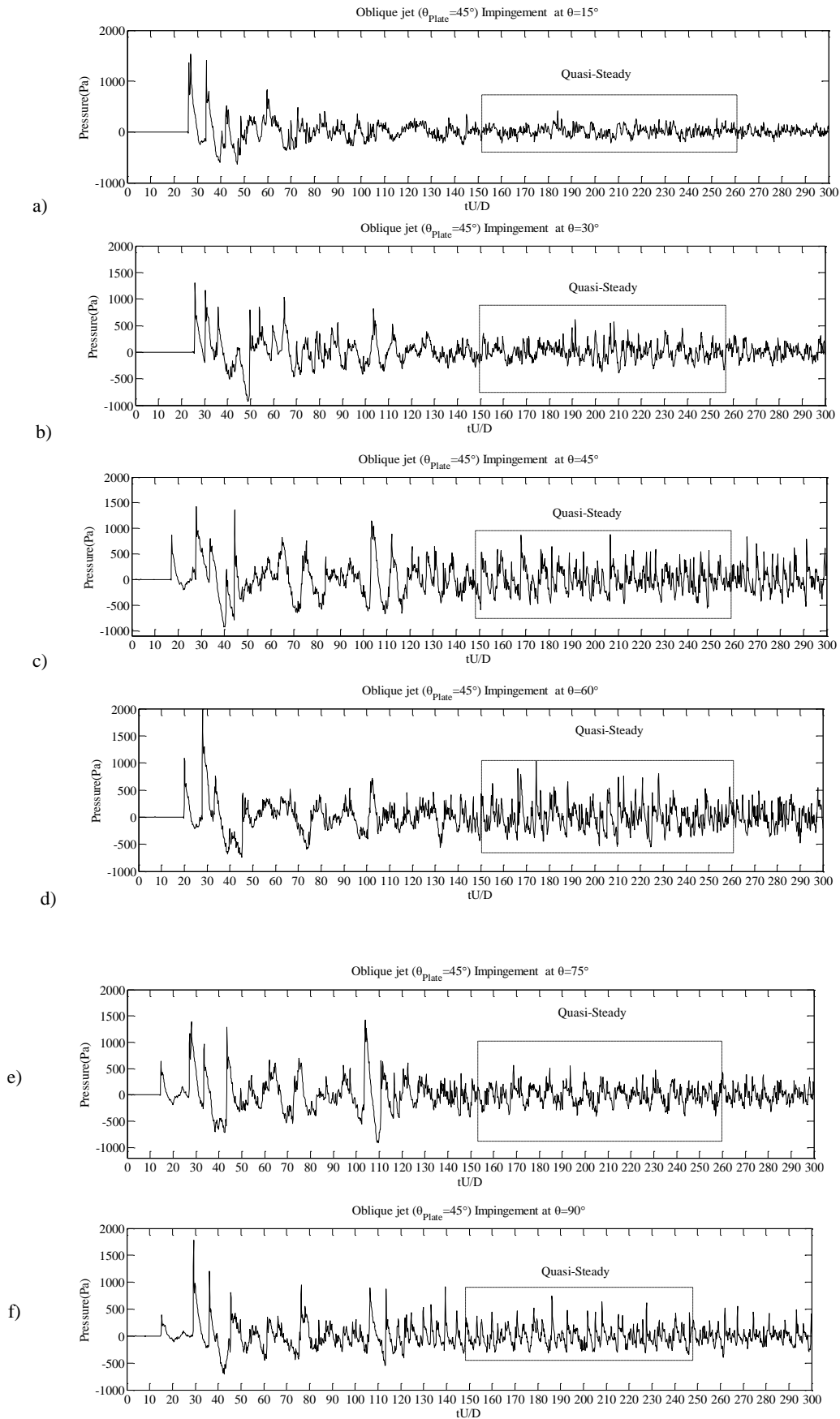
Fig. 6. The acoustic pressure signal for microphones at a) \theta=15^\circ , b) \theta=30^\circ , c) \theta=45^\circ , d) \theta=60^\circ , e) \theta=75^\circ , and f) \theta=90^\circ of the oblique jet impingement to a 45^\circ inclined plate.
