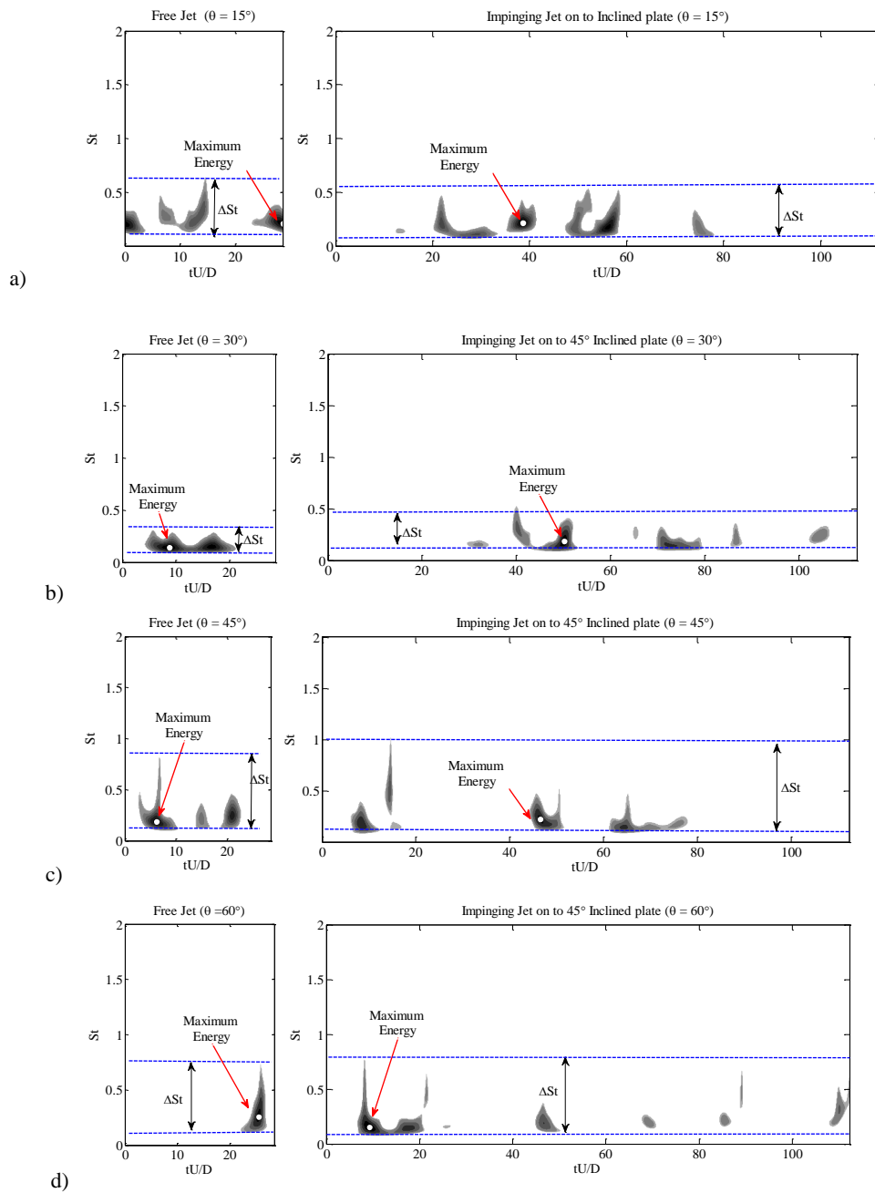
Fig. 8. Scalogram of acoustic pressure signal of quasi-steady free jet (left) and oblique jet impingement to a 45^\circ inclined plate (right) at a) \theta=15^\circ , b) \theta=30^\circ c) \theta=45^\circ d) \theta=60^\circ , e) \theta=75^\circ and f) \theta=90^\circ .
