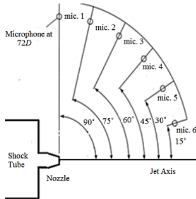
Fig. 2. Position of the microphones relative to the nozzle exit for the free jet.
