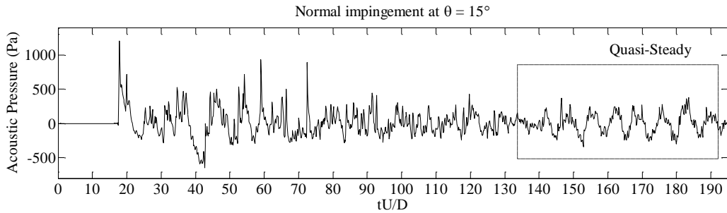
Fig. 10. Far-field acoustic pressure signal for the microphone positioned at \theta=15^\circ of normal jet impingement to the flat plate.
