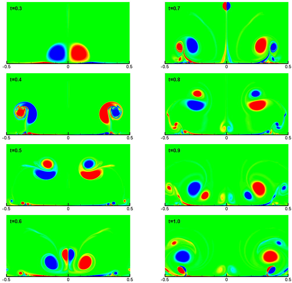
Fig. 2. Sequence of computed flowfield near the bottom wall shown by vorticity contours for dipole vorticity dynamics colliding with no-slip wall at Re = 10^4 .
