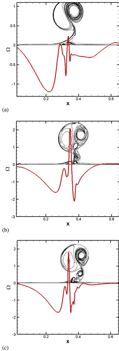
Fig. 5. Vorticity distribution on the bottom wall after dipole collision at t = 0.4 for (a) Re = 2 \times 10^4 , (b) Re = 5 \times 10^4 , and (c) Re = 10^5 .
