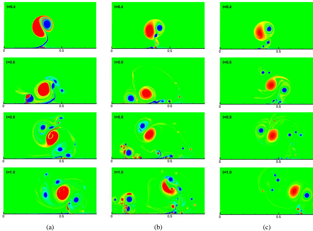
Fig. 4. Sequence of computed flowfield shown by vorticity contours for dipole vorticity dynamics colliding with no-slip wall at (a) Re = 2 \times 10^4 , (b) Re = 5 \times 10^4 , and (c) Re = 10^5 .
