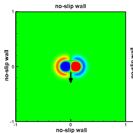
Fig. 1. Geometry and initial condition shown by vorticity field \Omega for studying the dipole vorticity dynamics colliding with the wall.
