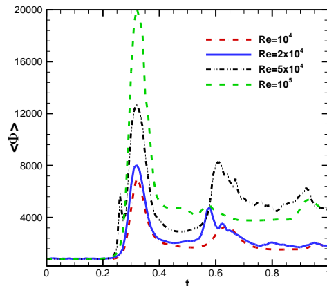
Fig. 6. Comparison of instantaneous averaged enstrophy in the flow domain for dipole vorticity dynamics colliding with no-slip wall.
