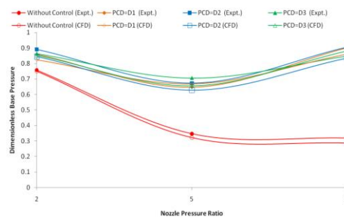
Fig. 17. P_b/P_a vs. NPR for M = 1.5 .
