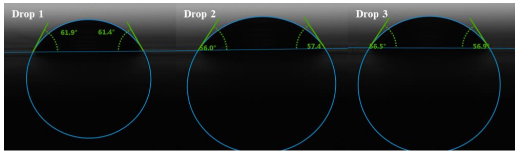
Fig. 5. Drop shape analysis for PMMA material.
