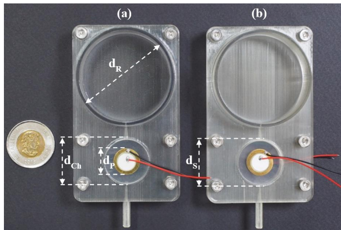
Fig. 2. Fabricated micropumps (a) SDM, (b) BDM.
