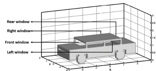
Fig. 4. Detailed configuration of the car model and four windows.
