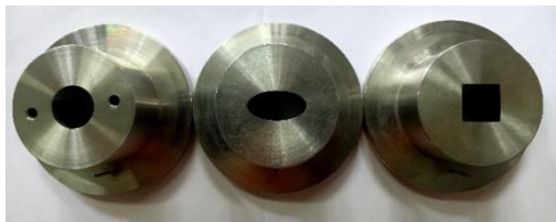
Fig. 4. Image of the circular, elliptic, and square nozzles.
