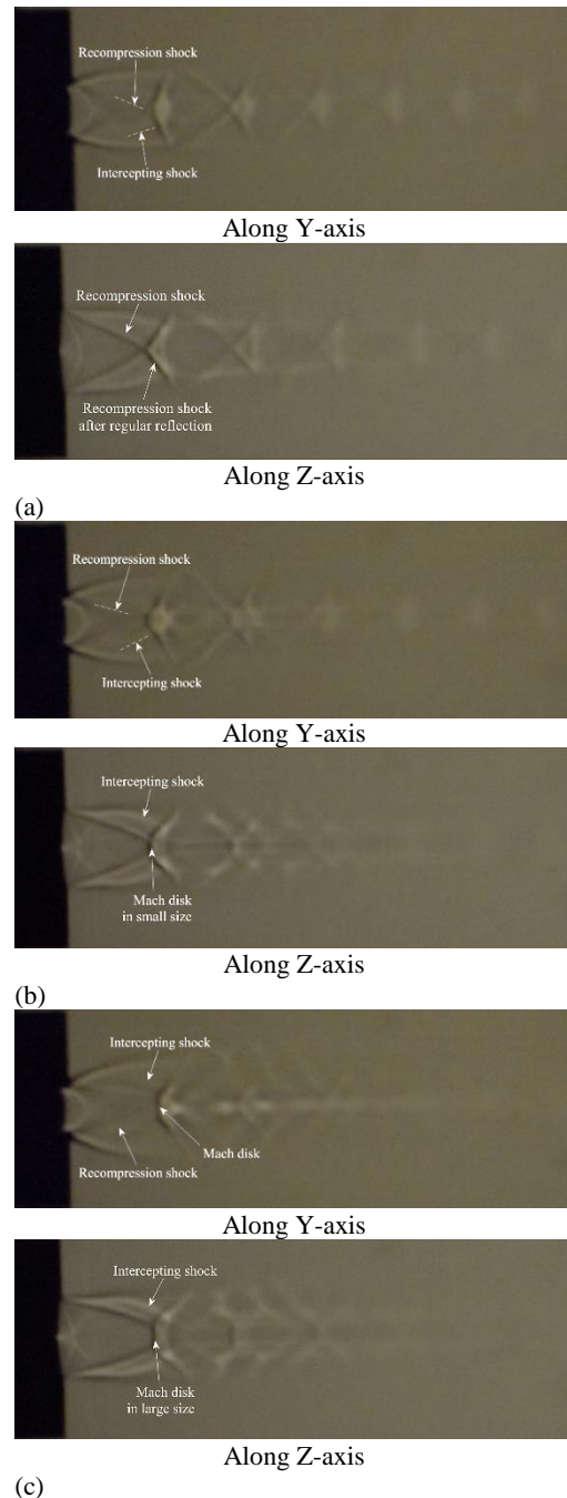
Fig. 9. Shadowgraph views of the square jet at (a) NPR 3 (b) NPR 4 (c) NPR 5.
