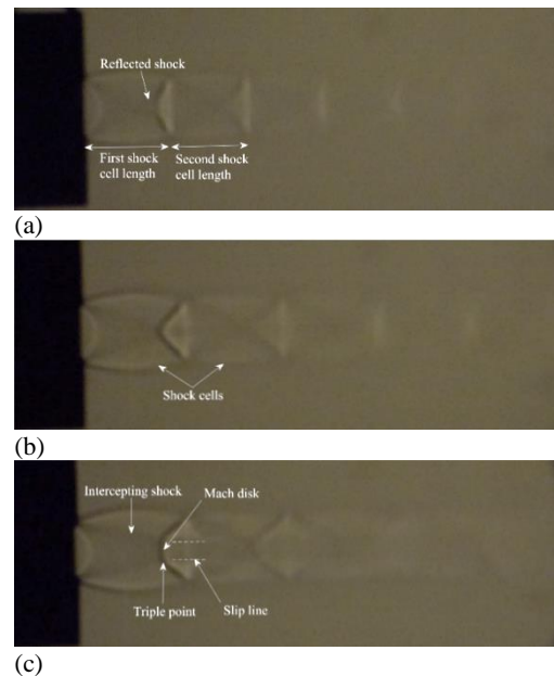
Fig. 7. Shadowgraph views of the circular jet at (a) NPR 3 (b) NPR 4 (c) NPR 5.
