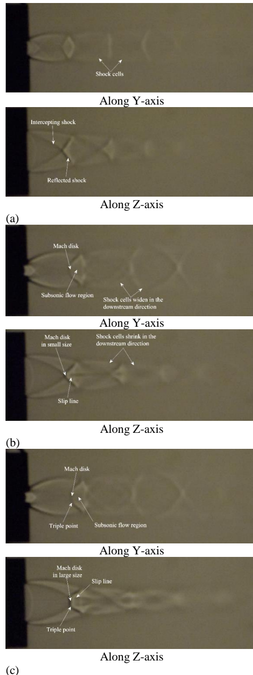
Fig. 8. Shadowgraph views of the elliptic jet at (a) NPR 3 (b) NPR 4 (c) NPR 5.
