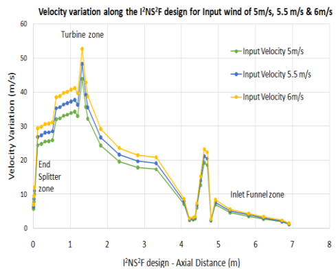
Fig. 26. Velocity variations for I 2 NS 2 F design for the input wind speed of 5m/s, 5.5m/s & 6m/s.
