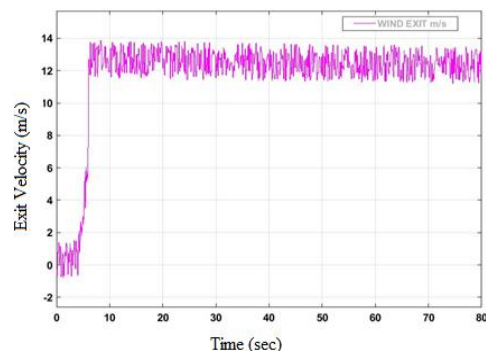
Fig. 17. Exit velocity.
