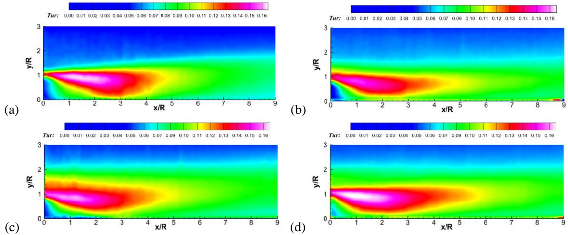
Fig. 6. Turbulence intensity nephogram of rough element wake: (a) Single-hemisphere rough element. (b) Double-hemisphere rough element with L = 3R . (c) Double-hemisphere rough element with L = 5R . (d) Double-hemisphere rough element with L = 7R .
