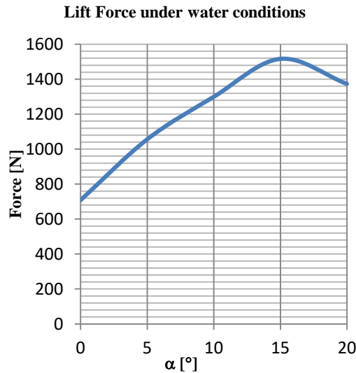
Fig. 12. Numerical lift for ceobtained under water conditions.
