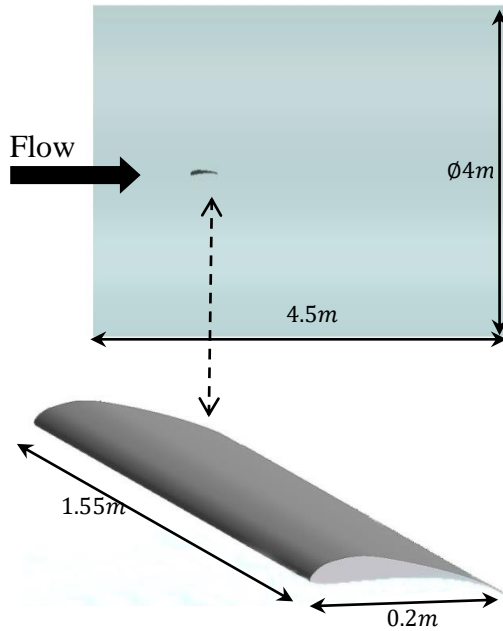
Fig. 5. Hydrofoil and 2-D diametral-plane scheme of the Volume of Control dimension of the 3-D numerical model geometry.
